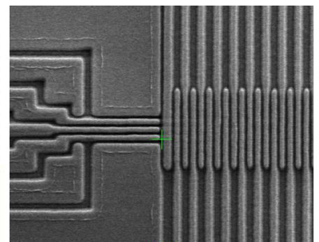
▲ Nanostructure as designed (left) and after e-beam nanopatterning and etching (right). Smallest pitch 80 nm, trench width 28 nm. In cooperation with Infineon Dresden, RWTH Aachen, and FZ Jülich.
